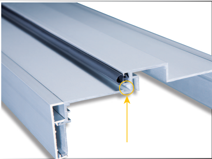
Concealed intumescent pocket eliminates the need for unsightly tape, or costly Category "A" constructed doors.
