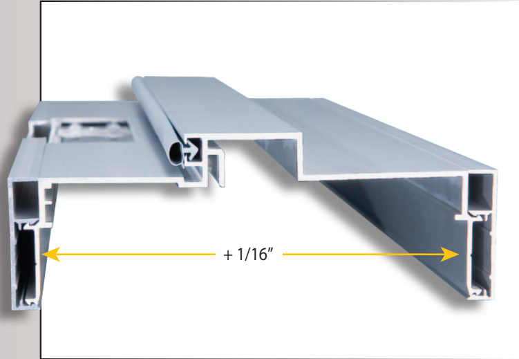
1/16" expanded throat makes installation easier.
